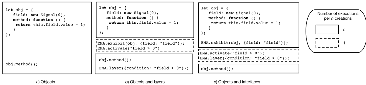
Fig. 10. Three pieces of code used for the EMAs performance evaluation: (a) Only creates objects, (b) creates objects and deploys layers, and (c) creates objects and interfaces.
